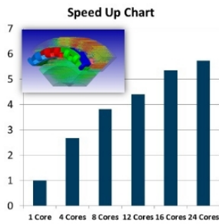
ANSYS Electronics HPC significantly accelerates an ANSYS Maxwell 3-D Transient simulation of an electric motor.
